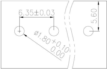
PCB LAYOUT
