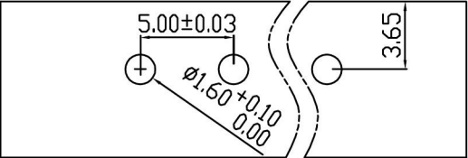
PCB LAYOUT
